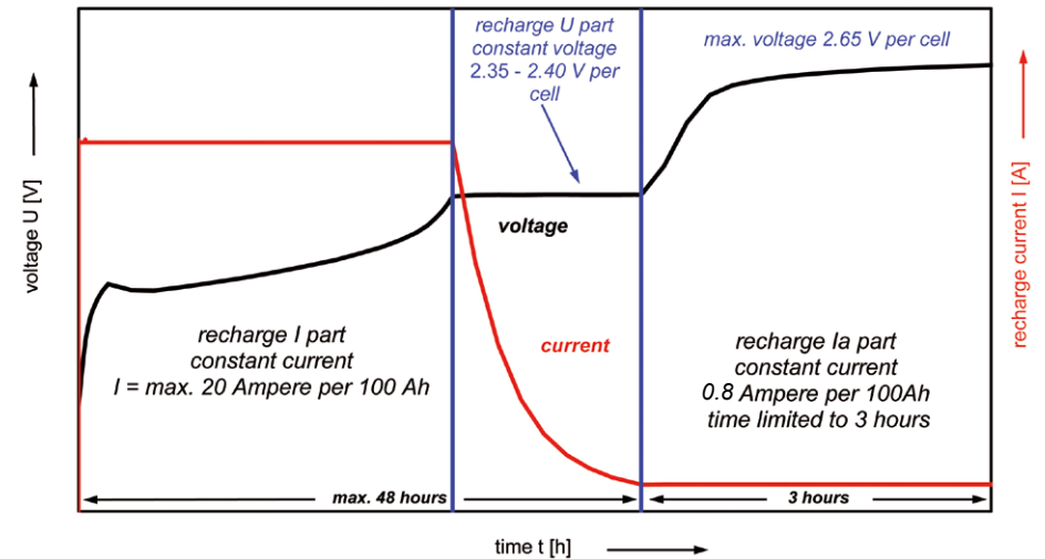
Fig. 9-2: IUa characteristic
